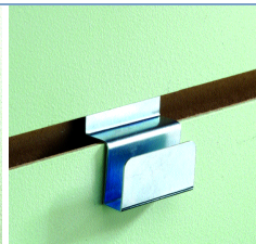
06-6068 Frame slatwall hanger Galvanized steel
